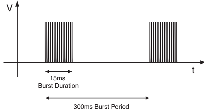
Figure 2-2. Fast Transient Burst
