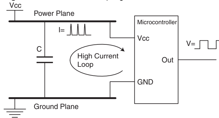
Figure 4-1. Incorrect Decoupling
